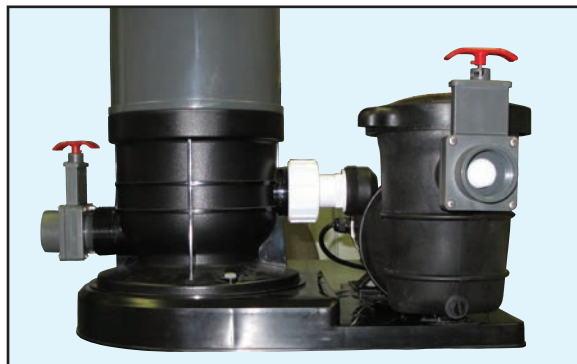
4B – Plastic pump housing mount
