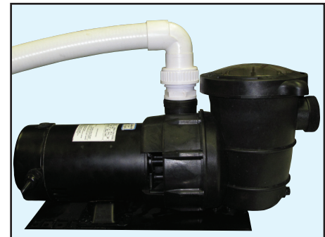
Figure 22 — Attaching flex pipe to pump
