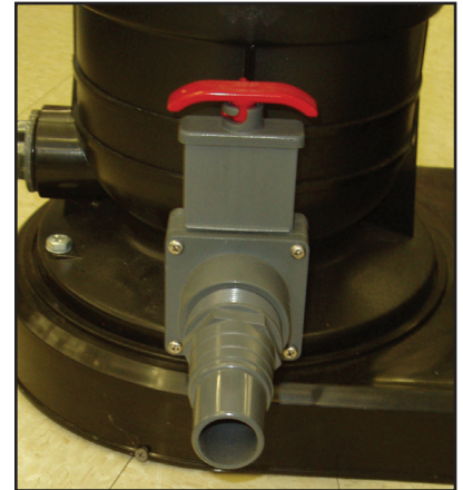
Figure 1 – Slide valve attached "TO POOL" on tank
